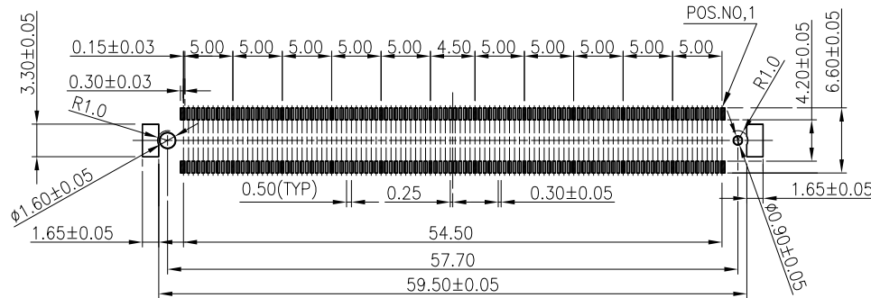
REFERENCE PCB LAYOUT
